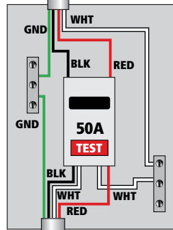
50 AMP GFCI
